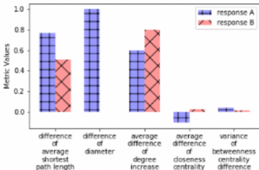
Figure 3: Changes of network indices after merging assessment knowledge with two responses
