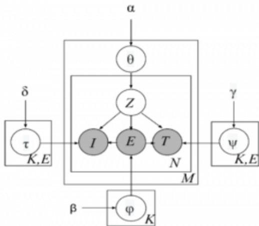
Figure 1: Plate notation for HBTM
